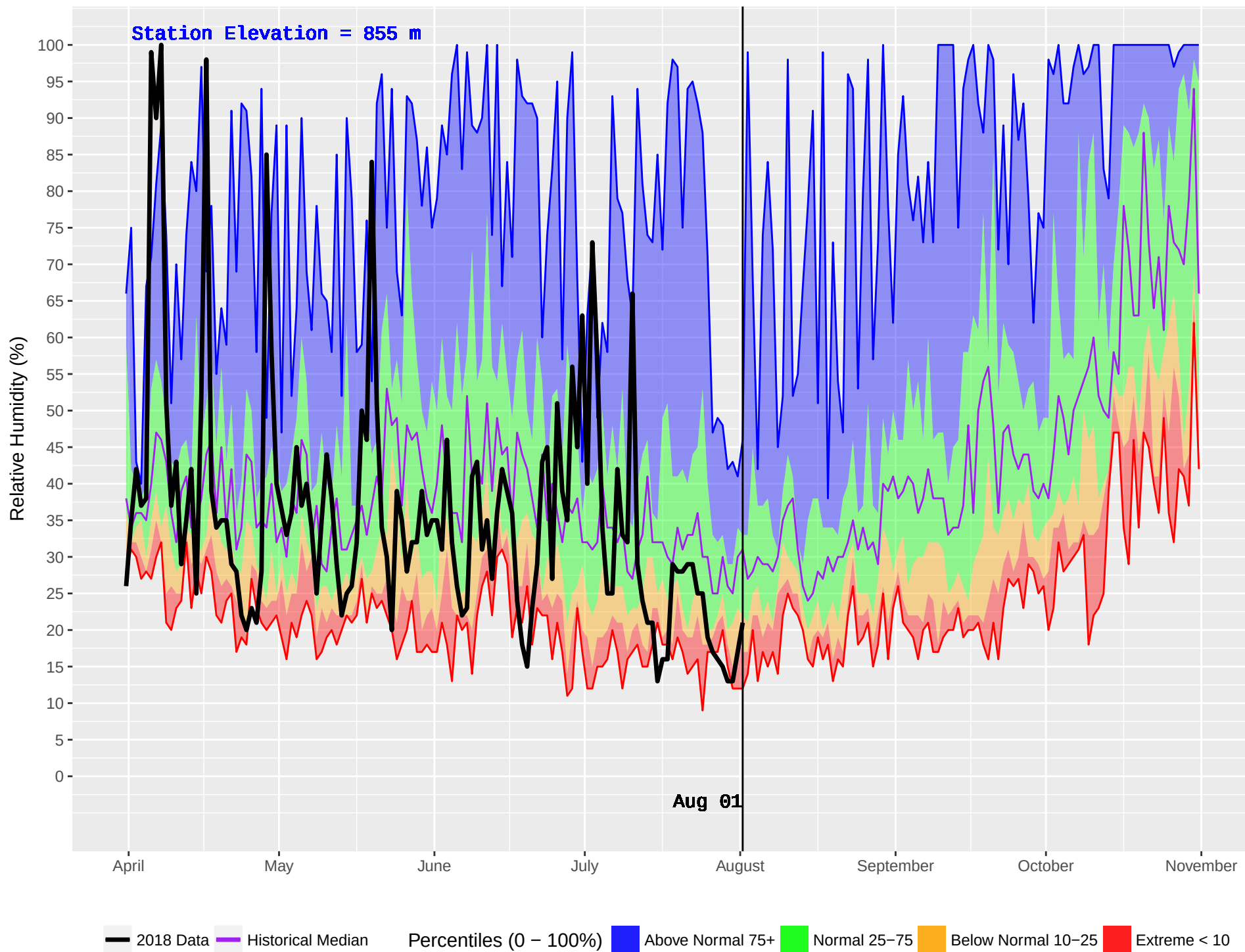
AUGUST LAKE (836) : Historical (2003–2016) and Current (2018) Daily Relative Humidity
