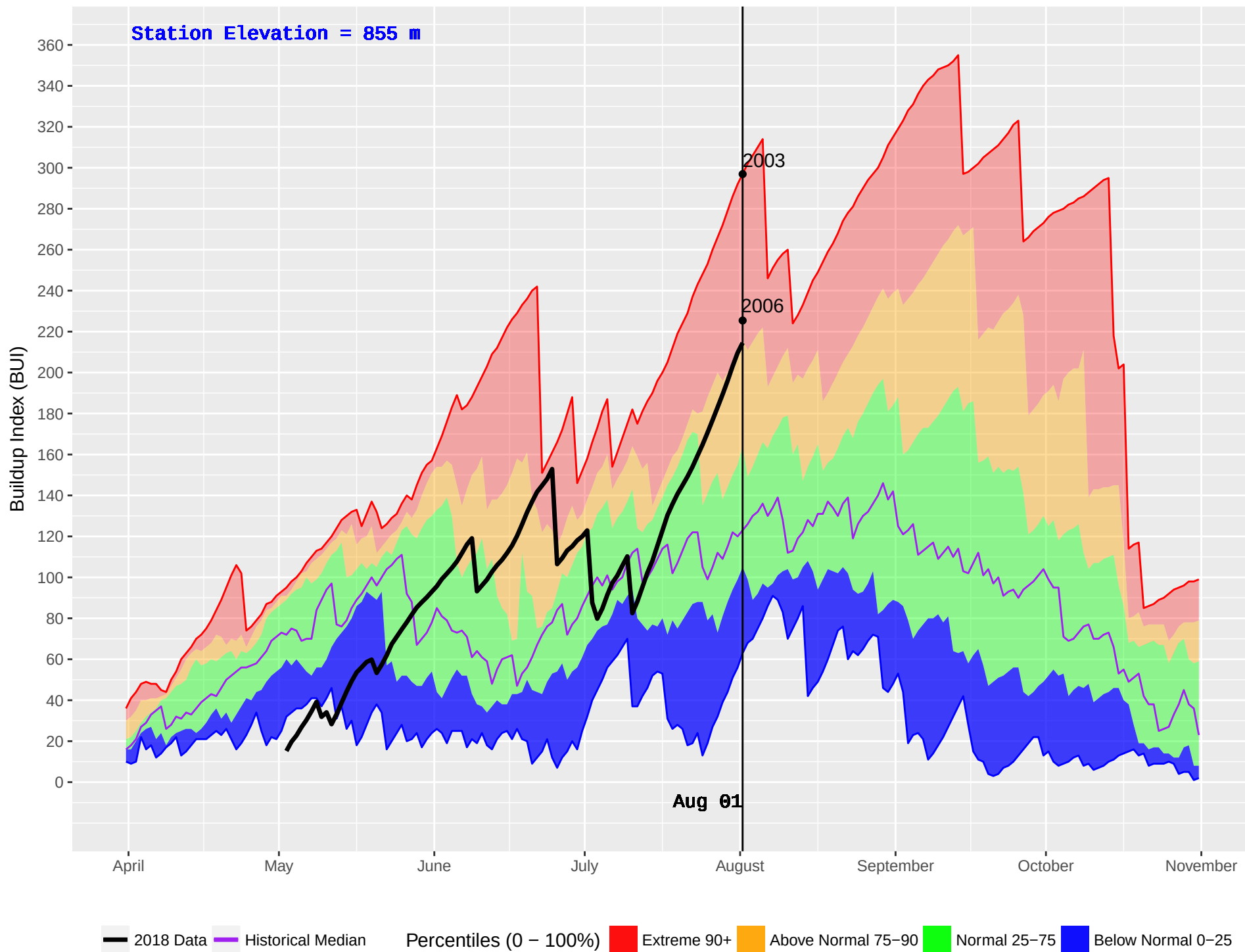
AUGUST LAKE (836) : Historical (2003–2016) and Current (2018) Daily Buildup Index (BUI)
