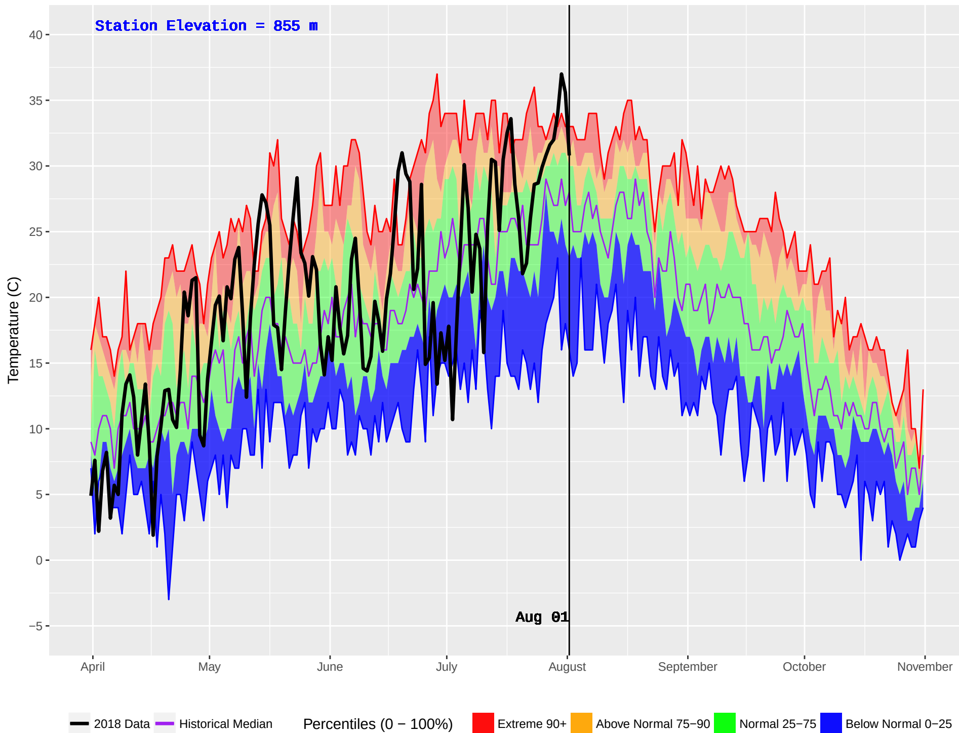
AUGUST LAKE (836) : Historical (2003–2016) and Current (2018) Daily Temperature
