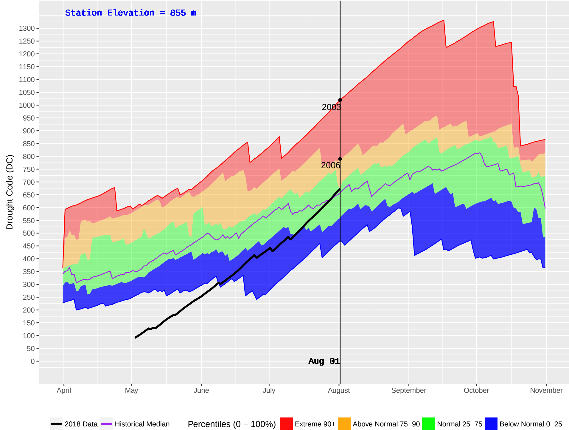
AUGUST LAKE (836) : Historical (2003–2016) and Current (2018) Daily Drought Code (DC)
